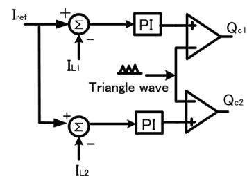
Fig. 8. Controller diagram of chopper circuit
