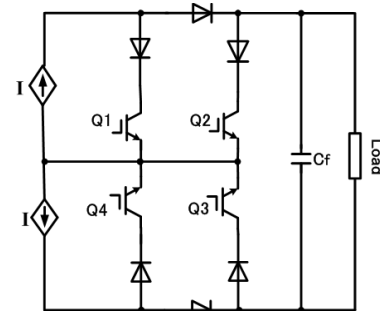
Fig. 1. Fundamental three-level CSI
