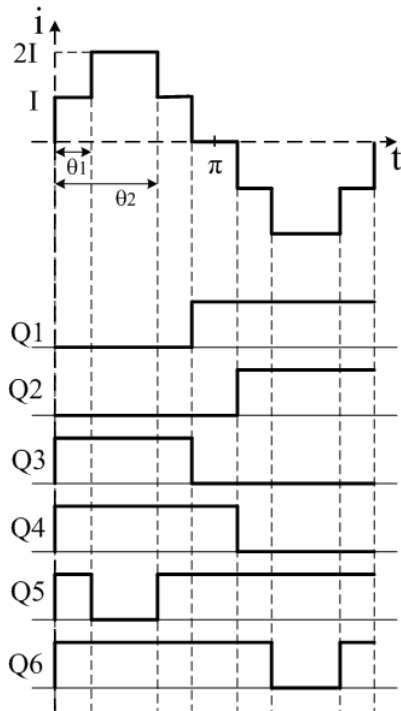
Fig. 5. Five-level current waveform generation
