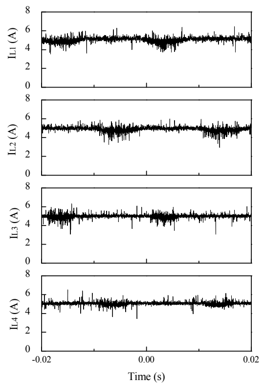
(b) Waveforms of DC current sources Fig. 13. Experimental waveforms
