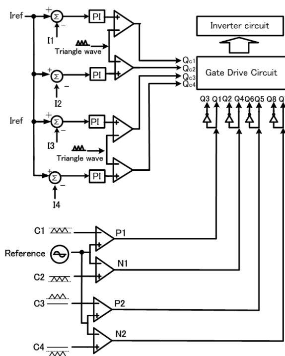
Fig. 11. Controller diagram of five-level CSI
