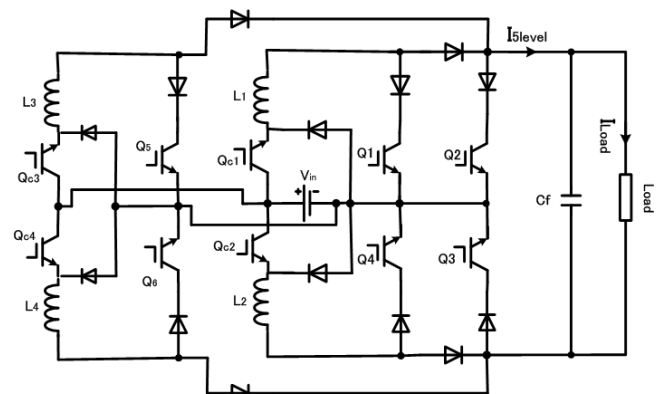
Fig. 9. Simulation and experimental test circuit of five-level CSI
