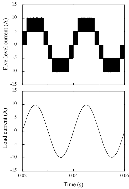
(a) Five-level and load currents
