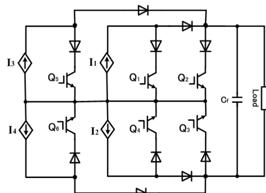
Fig. 4. Five-level CSI circuit ( I_1=I_2=I_3=I_4=I )
