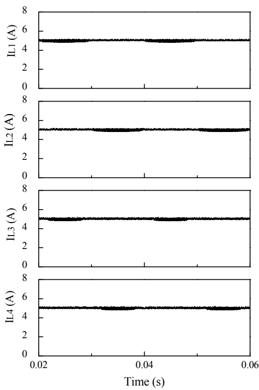
(b) Waveforms of DC current sources Fig. 12. Simulation waveforms
