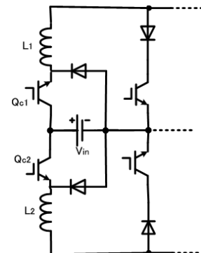
Fig. 7. Two-level CSI module with chopper circuit
