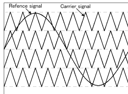
Fig. 10. Multi-carrier based sinusoidal PWM
