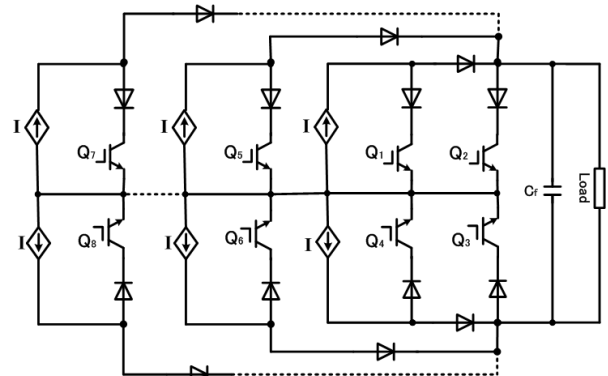
Fig. 3. Generalized configuration of proposed multilevel CSI
