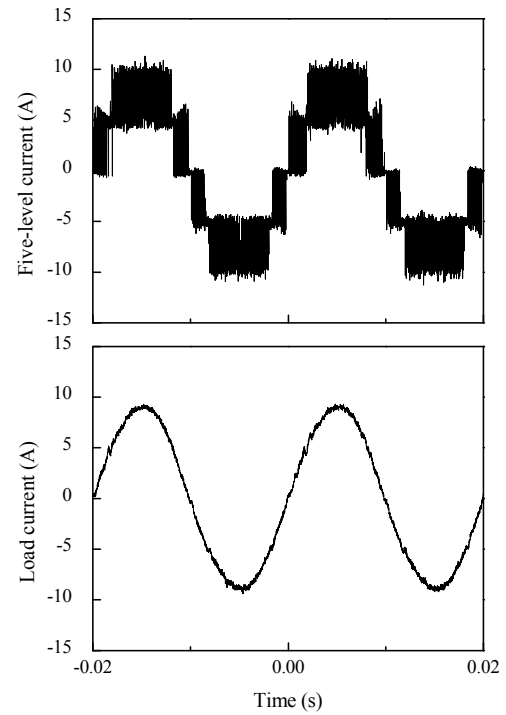
(a) Five-level and load currents
